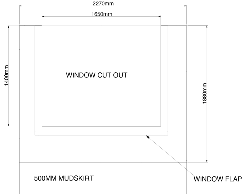
2M SWING AWN WINDOW WALL
